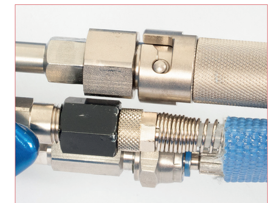
Quick release fastener in detail
